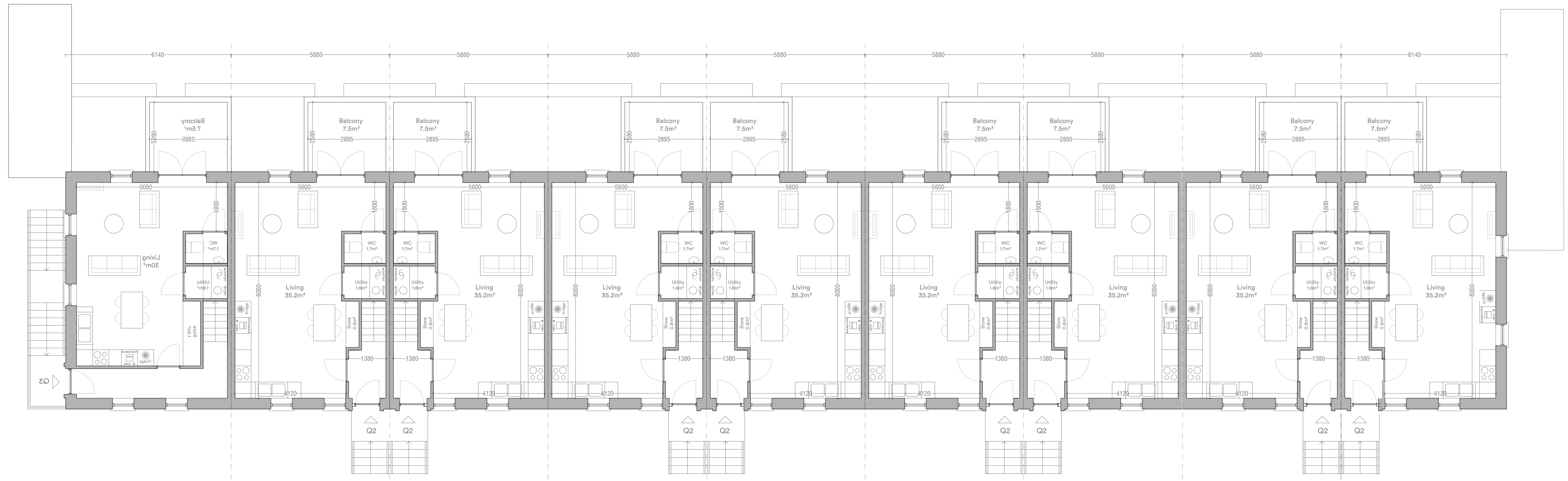
Duplex Block A First Floor
